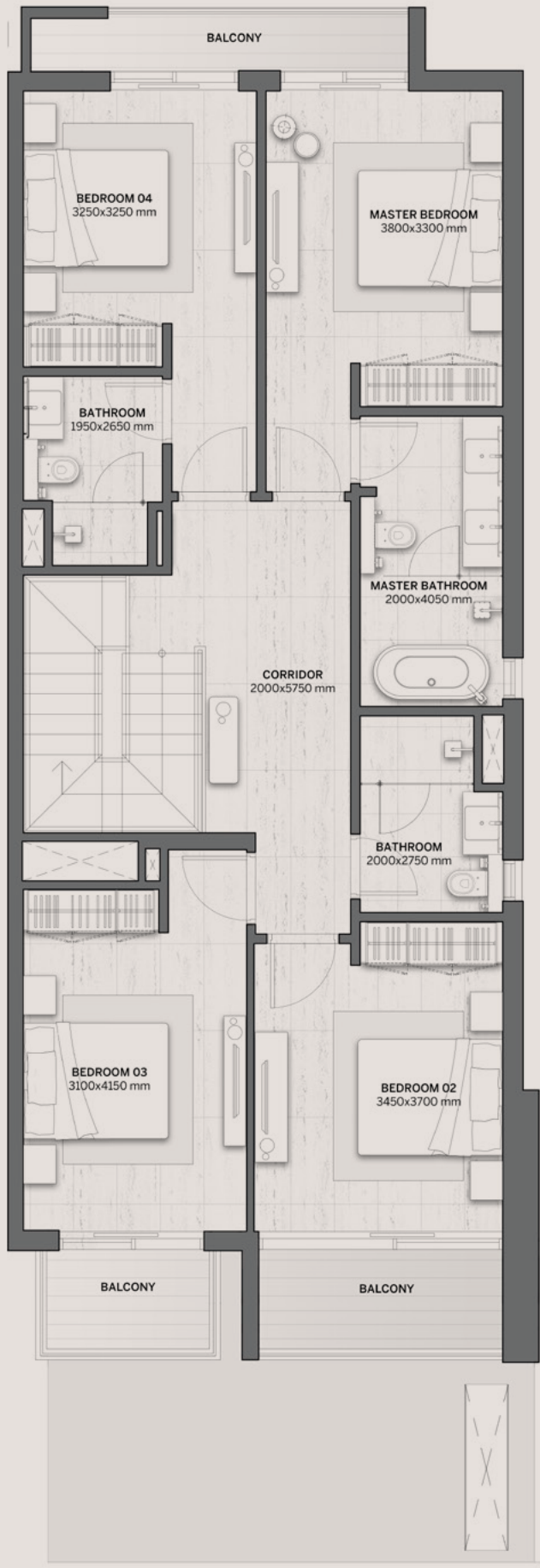
FIRST FLOOR
