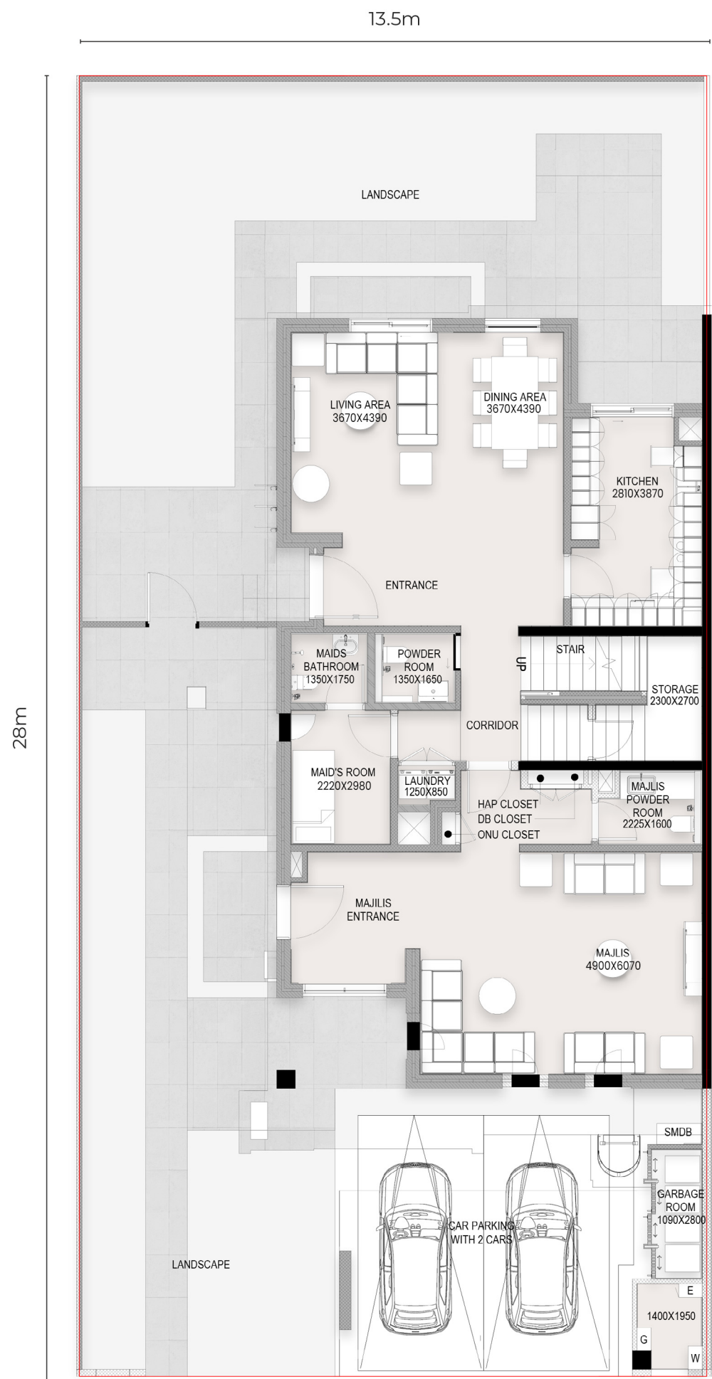
GROUND FLOOR
