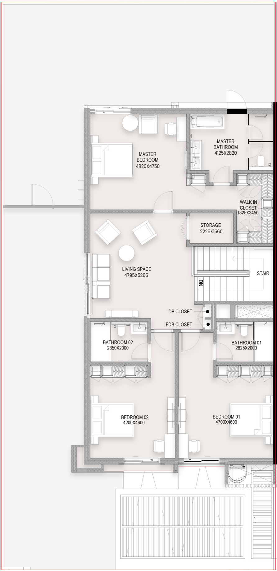
FIRST FLOOR
