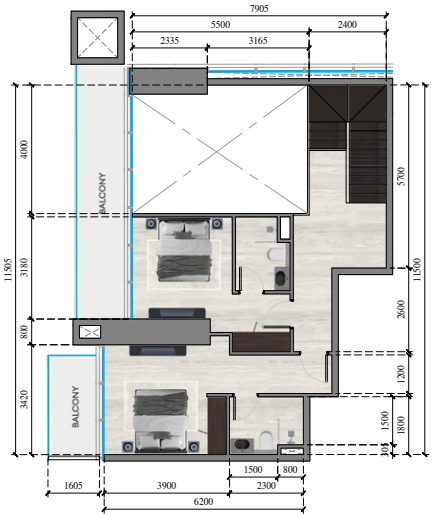
FIRST FLOOR LEVEL
